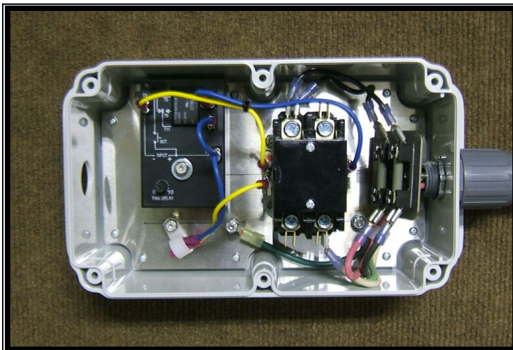
Inside view of electrical enclosure
